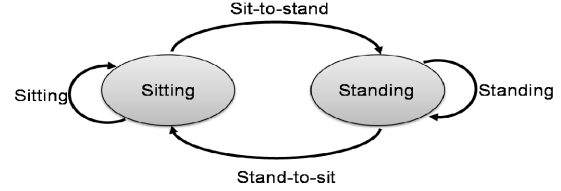
Figure 4. Finite state machine (FSM) model. Ellipses: states (i.e. tasks). Arrows: transitions between tasks.
