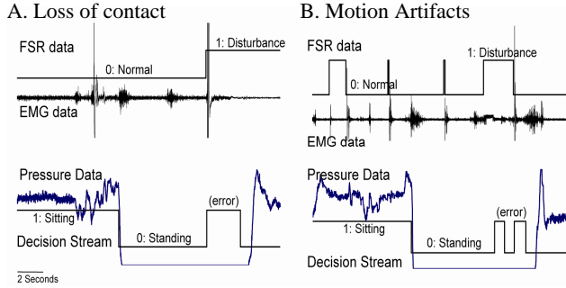
Figure 7. Offline performance of EMG pattern classifier under two disturbances: (A) loss of electrode contact and (B) motion artifacts. The EMG signals under disturbances are demonstrated. The timings when the disturbances were introduced are indicated by FSR data (0: normal; 1: under disturbance). The output decisions (0: standing; 1: sitting) are aligned with the pressure data (the lower panels).
